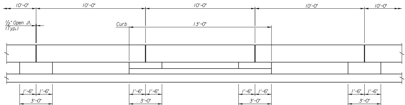
PARTIAL CORRAL RAIL ELEVATION (Along Traffic Face, West Corral Rail shown, East Corral Rail similar) Showing curb above Pier #2 and Pier #4
