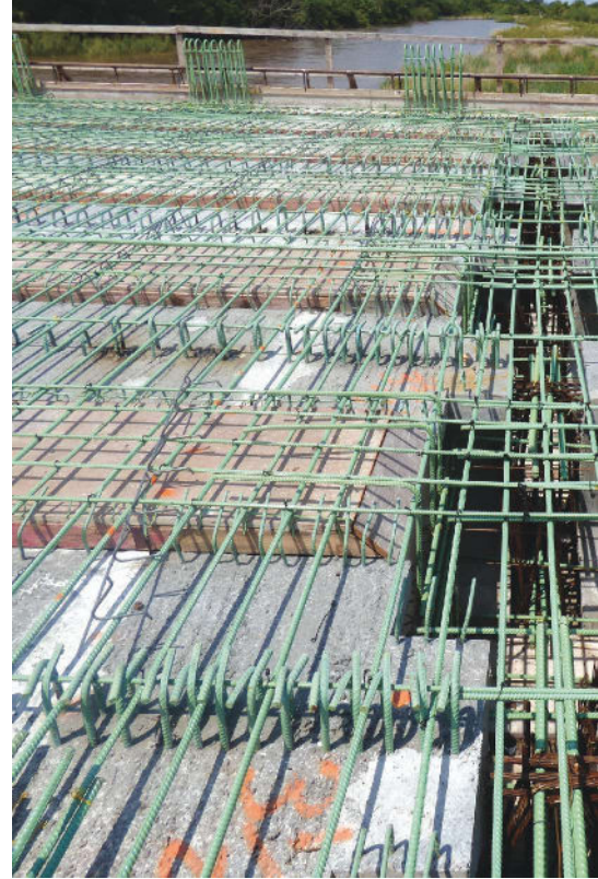
All reinforcement in the superstructure was epoxy-coated.
