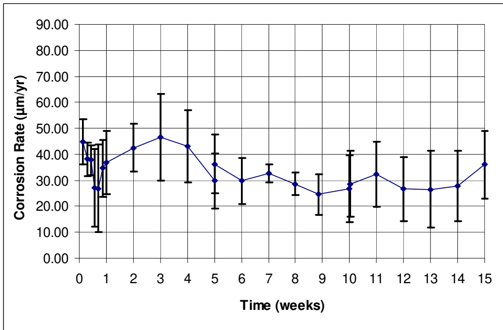
Figure 6: Average corrosion rate of conventional steel, Specimens 1-6.
