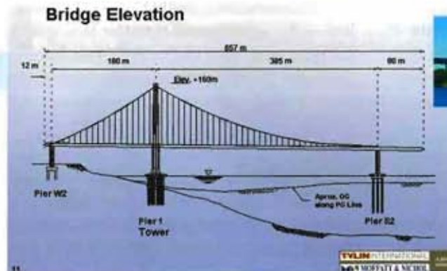
The new bridge concept
